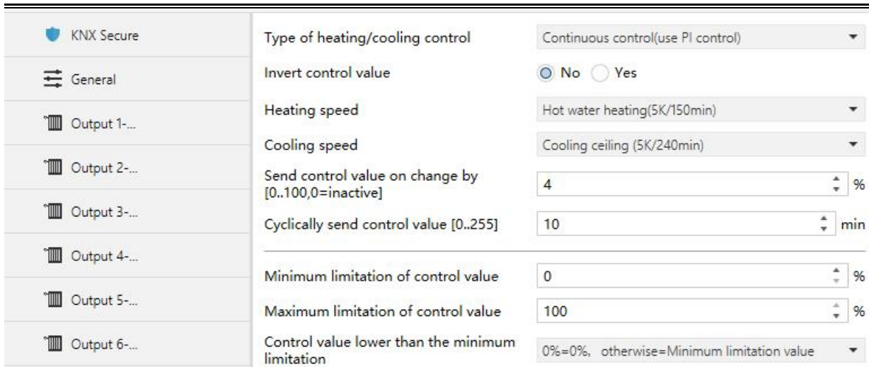
“Continuous control(use PI control)”参数设置
